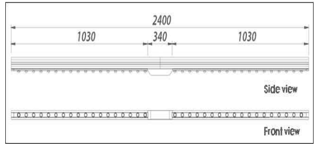
Fig. 4. Longitudinal Section on TD LED Lighting Fixture
