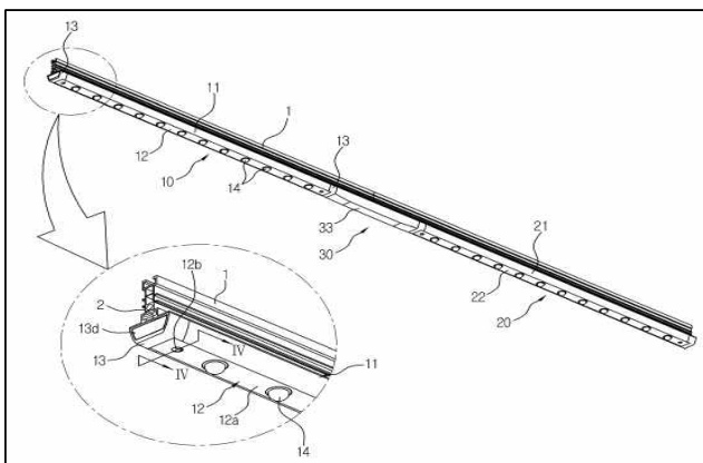
Fig. 6. Perspective on Patented TD LED Lighting Fixture
