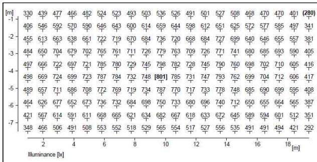
Fig. 9. Illumination Distribution at Display Module Line
