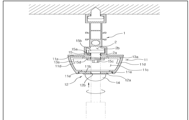
Fig. 7. Cross Section on Patented TD LED Lighting Fixture(Line IV~IV on Fig. 6)
