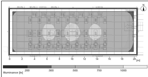
Fig. 8. Illumination Simulation at Display Module Line
