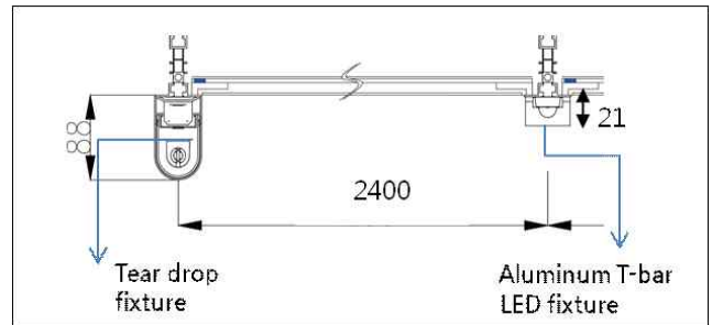
Fig. 5. Cross Section on TD LED Lighting Fixture
